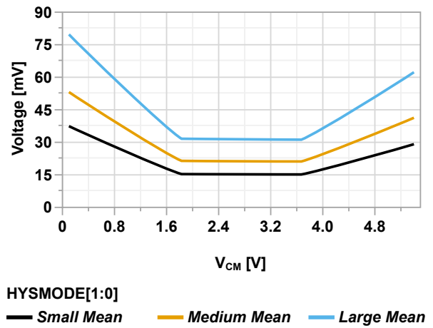
Figure 49-112. Input Hysteresis vs. Common Mode Voltage ( V_{DD} = 5.5V )
