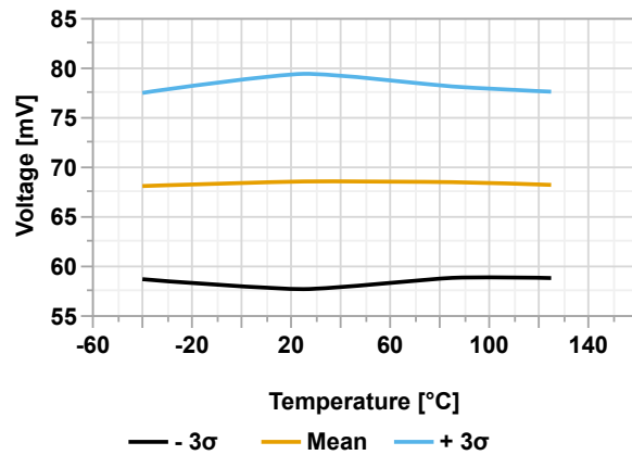
Figure 49-53. BOR Hysteresis (BORV[1:0] = 0x1) vs. Temperature
