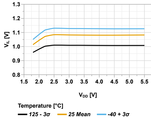
Figure 49-69. Input Pin with SMBus - Maximum V_{IL} vs. V_{DD}
