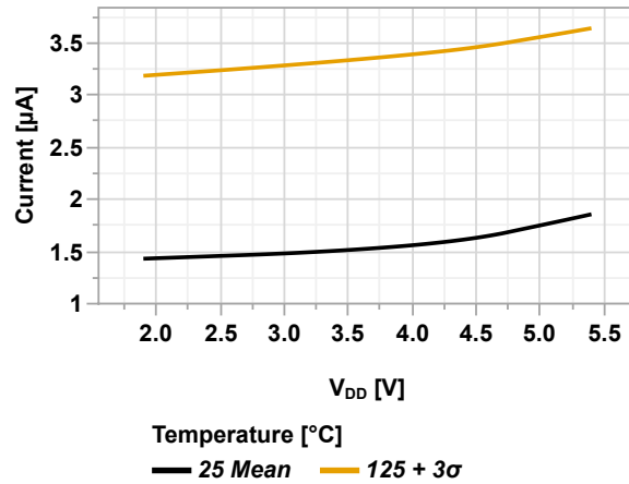
Figure 49-19. I_{PD} SOSC (SOSCPWR = Low Power) vs. V_{DD}
