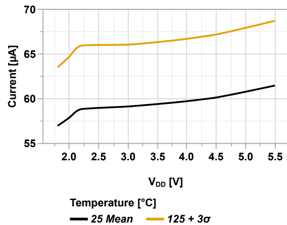
Figure 49-23. I_{PD} CDAFVR vs. V_{DD}
