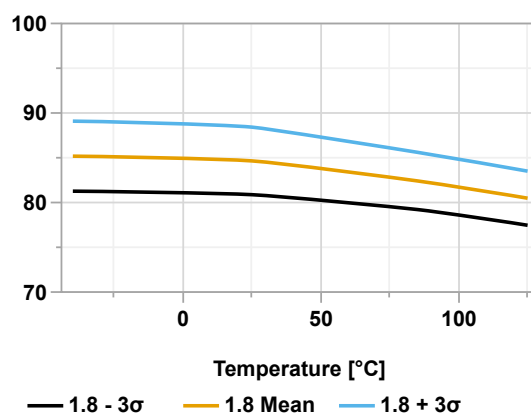
Figure 49-75. Weak Pull-up Current V_{SS} Temperature at V_{DD} = 5.0V
