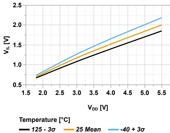
Figure 49-71. Reset Pin V_{IL} vs. V_{DD}
