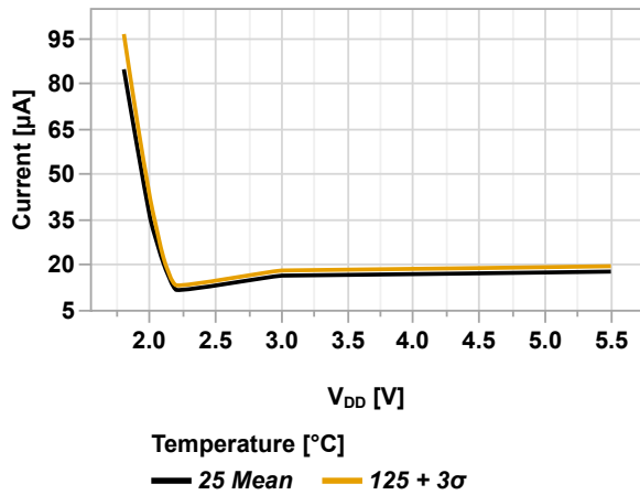
Figure 49-26. I_{PD} CMP (SP[1:0] = 0x0) vs. V_{DD}
