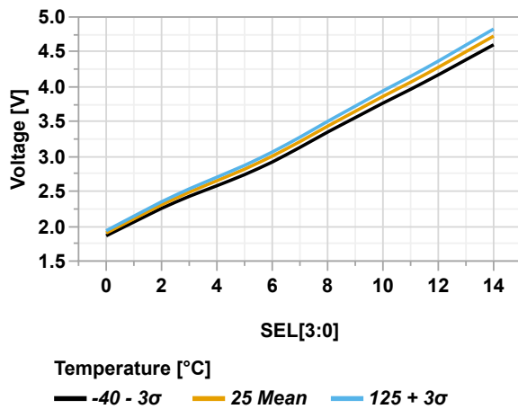
Figure 49-58. HLVD Negative Edge SEL[3:0] vs. Temperature
