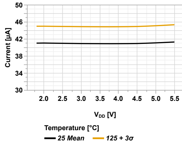
Figure 49-27. I_{PD} CMP (SP[1:0] = 0x1) vs. V_{DD}
