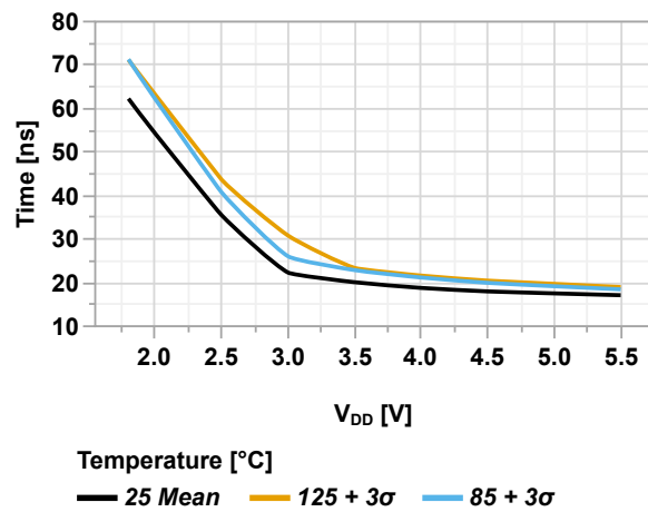
Figure 49-63. Rise Time (SLRxn = 0) vs. V_{DD}
