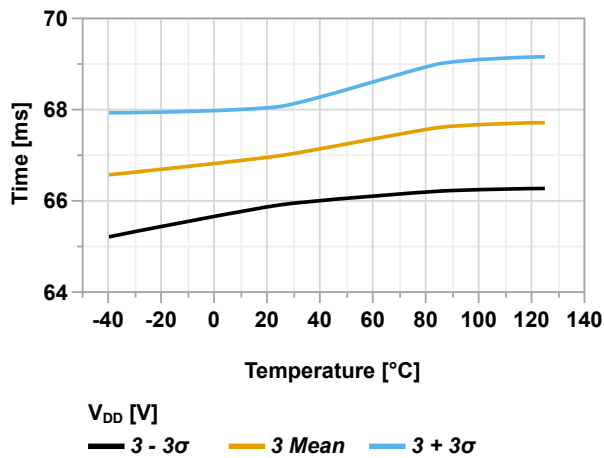
Figure 49-44. Start-up Time vs. Temperature (PWRTS[1:0] = 0x2, V_{DD} = 3.0V)
