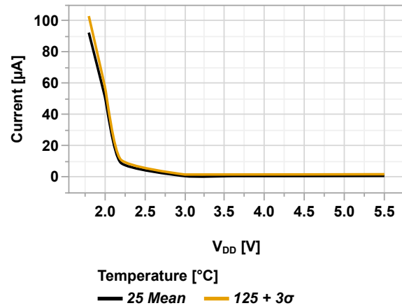
Figure 49-23. I_{PD} CDAFVR vs. V_{DD}
