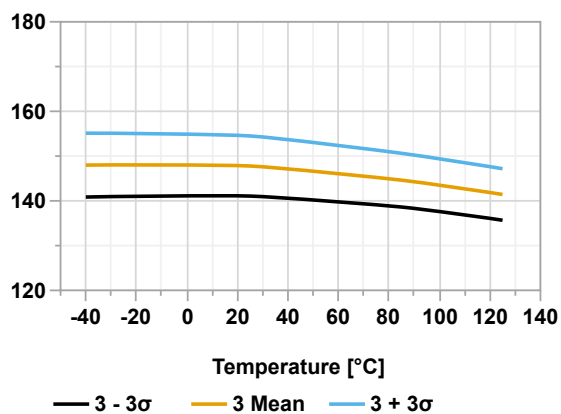
Figure 49-74. Weak Pull-up Current V_{SS} Temperature at V_{DD} = 3.0V
