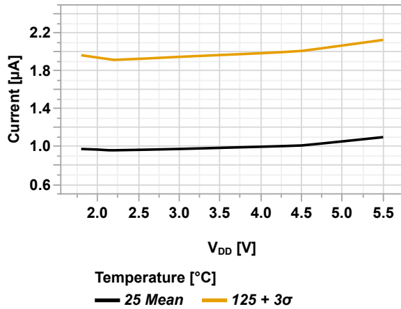
Figure 49-18. I_{PD} WDT vs. V_{DD}
