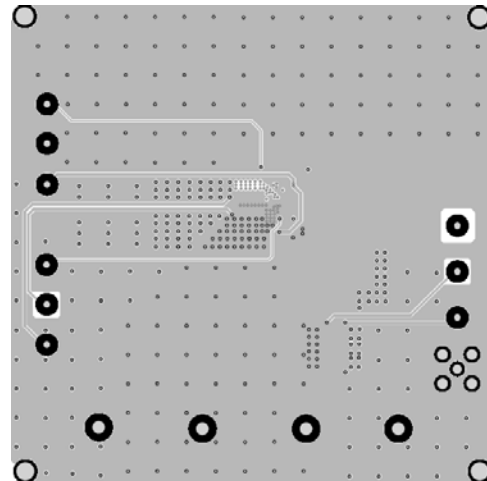
Figure 4: Inner Layer2
