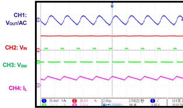
Steady State I_{OUT} = 3A
