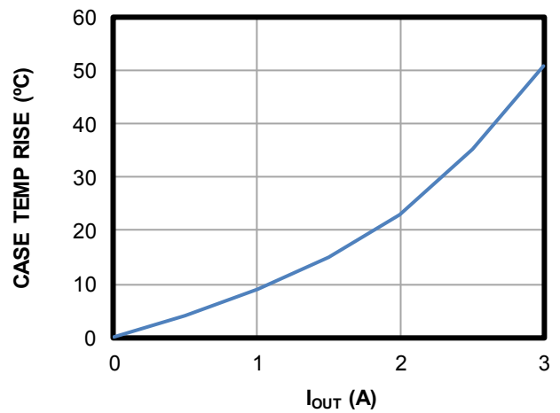
Case Temperature Rise vs. I_{OUT}
