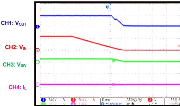
Input Power Shutdown I_{OUT} = 0A
