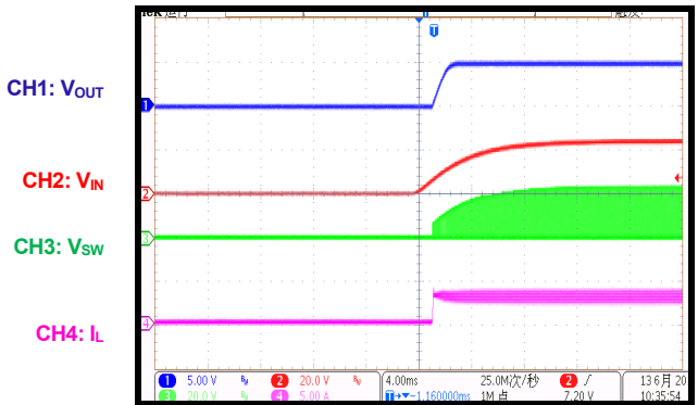
Input Power Start-Up I_{OUT} = 3A
