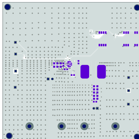
Figure 3: Top Layer
