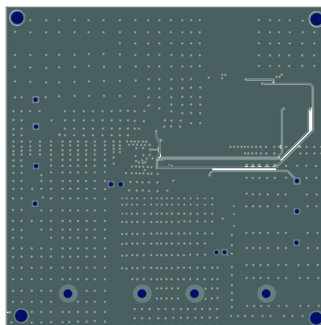
Figure 5: Mid-Layer 2
