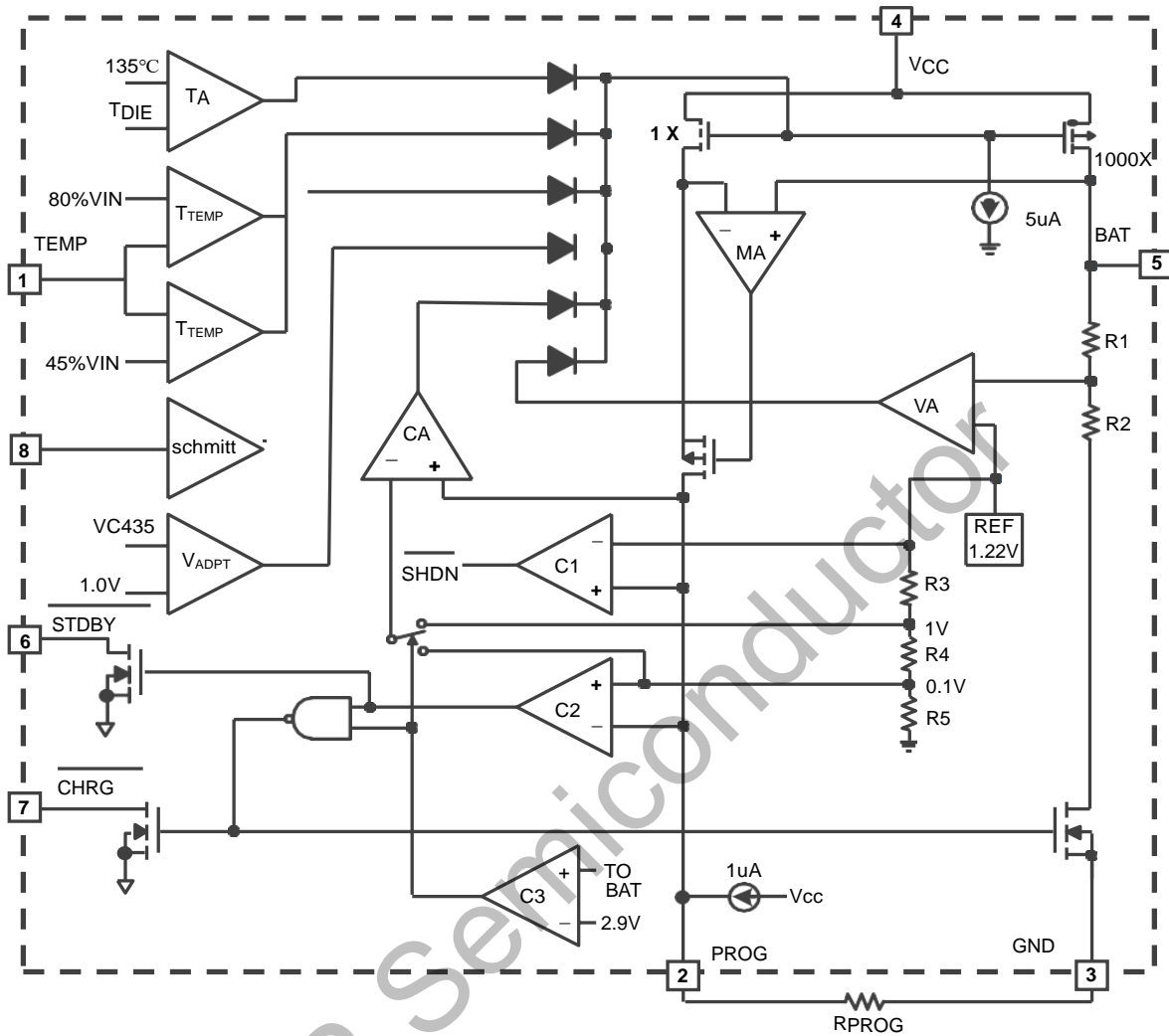
Figure 2. TP4056 Block Diagram
