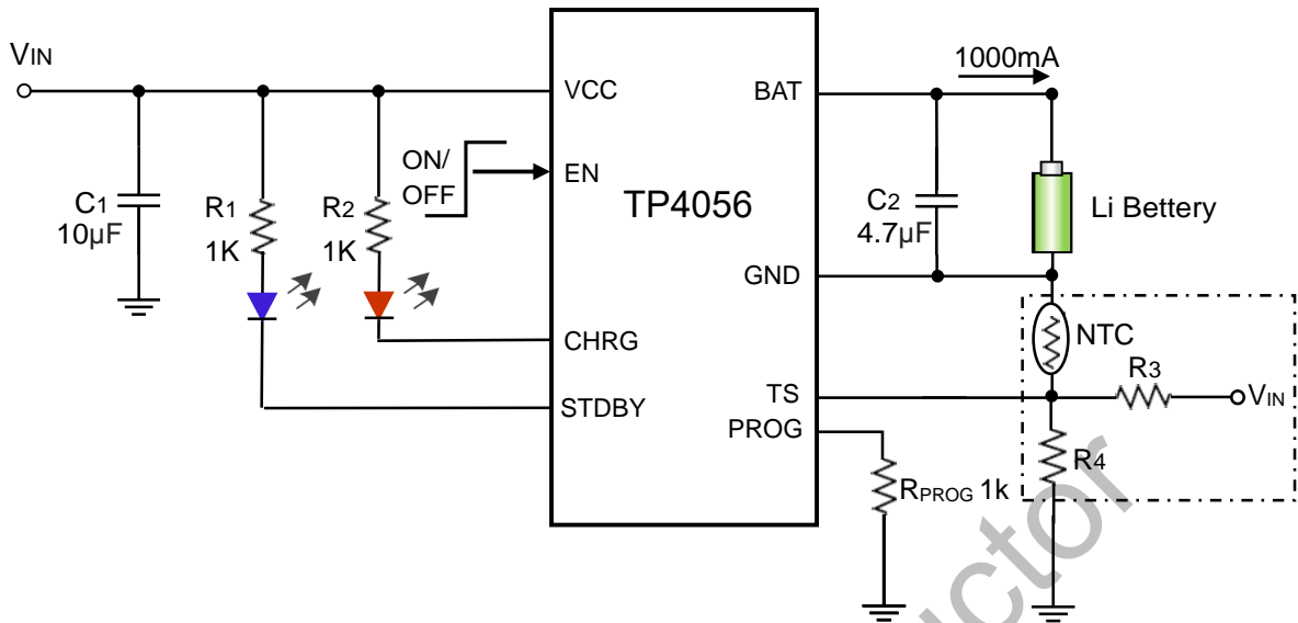
Figure 1. TP4056 Typical Application Circuit
