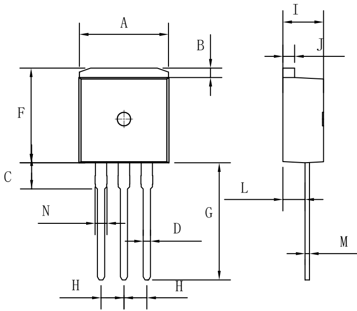
TO-262
