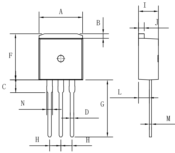
TO-262
