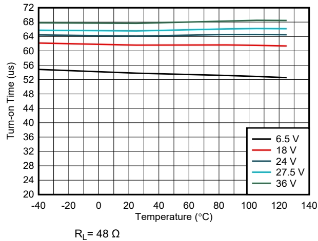
Figure 6-9. Turn-on Time ( t_{ON} ) vs Temperature vs VS Voltage
