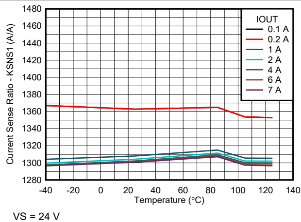
Figure 6-13. Current Sense Ratio (KSNS) vs Temperature vs Load Current
