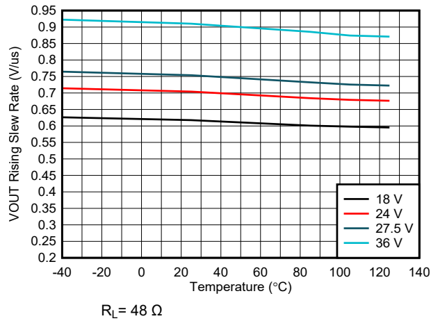
Figure 6-11. VOUT Rising Slew Rate ( SR_R ) vs Temperature vs VS Voltage
