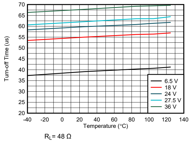
Figure 6-10. Turn-off Time ( t_{OFF} ) vs Temperature vs VS Voltage
