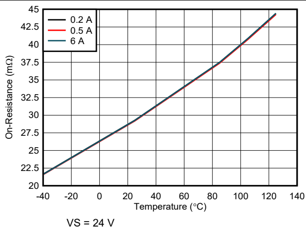
Figure 6-4. On-Resistance ( R_{ON} ) vs Temperature vs Load Current
