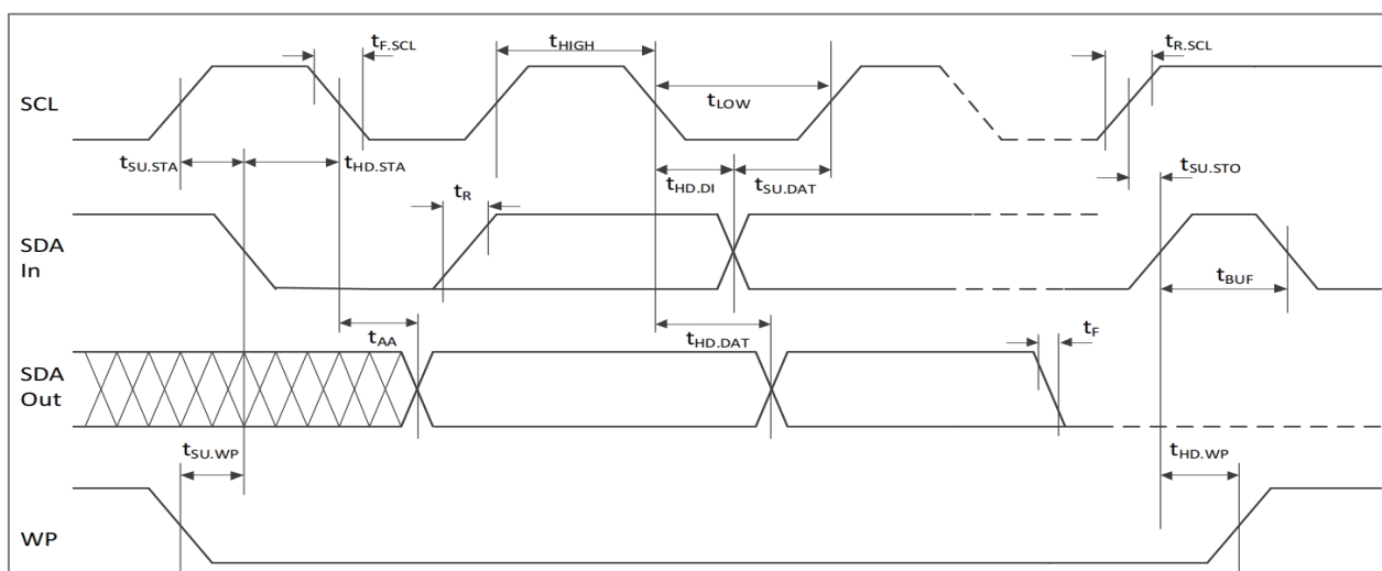
Figure 20 Bus Timing
