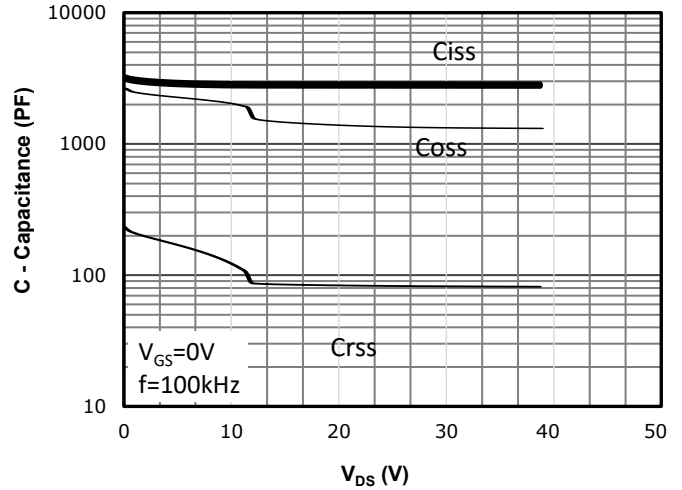
Fig 8: Capacitance Characteristics
