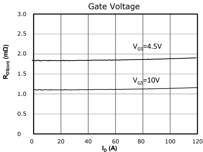
Fig 3: Rds(on) vs Drain Current and
