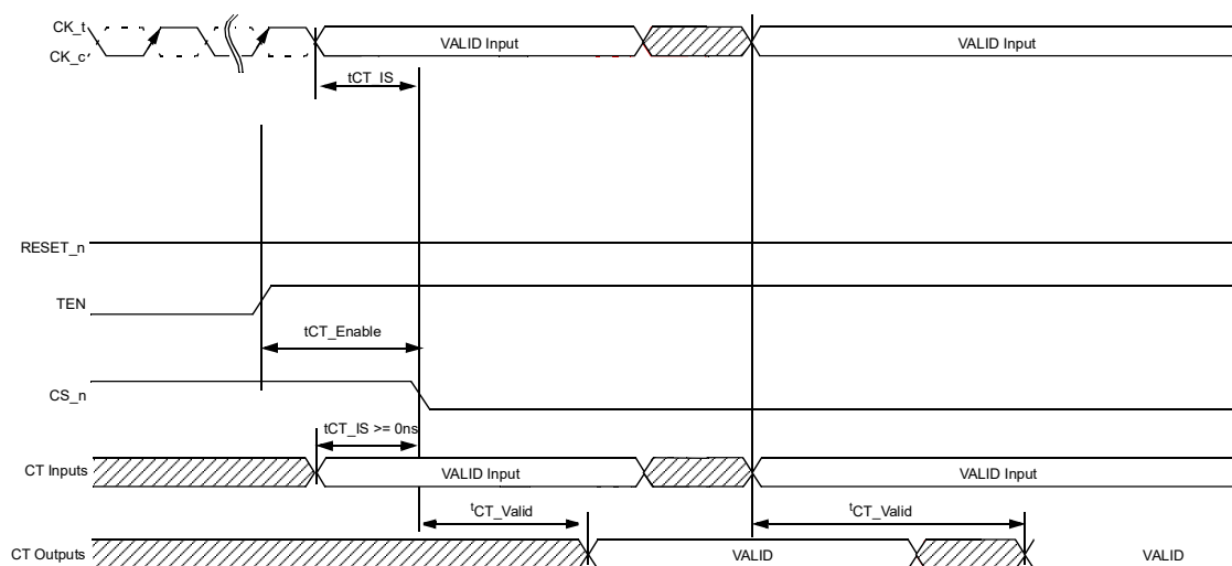
Figure 215 — Timing Diagram for Connectivity Test (CT) Mode
