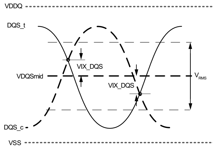
Figure 209 — VIX Definition (DQS)
