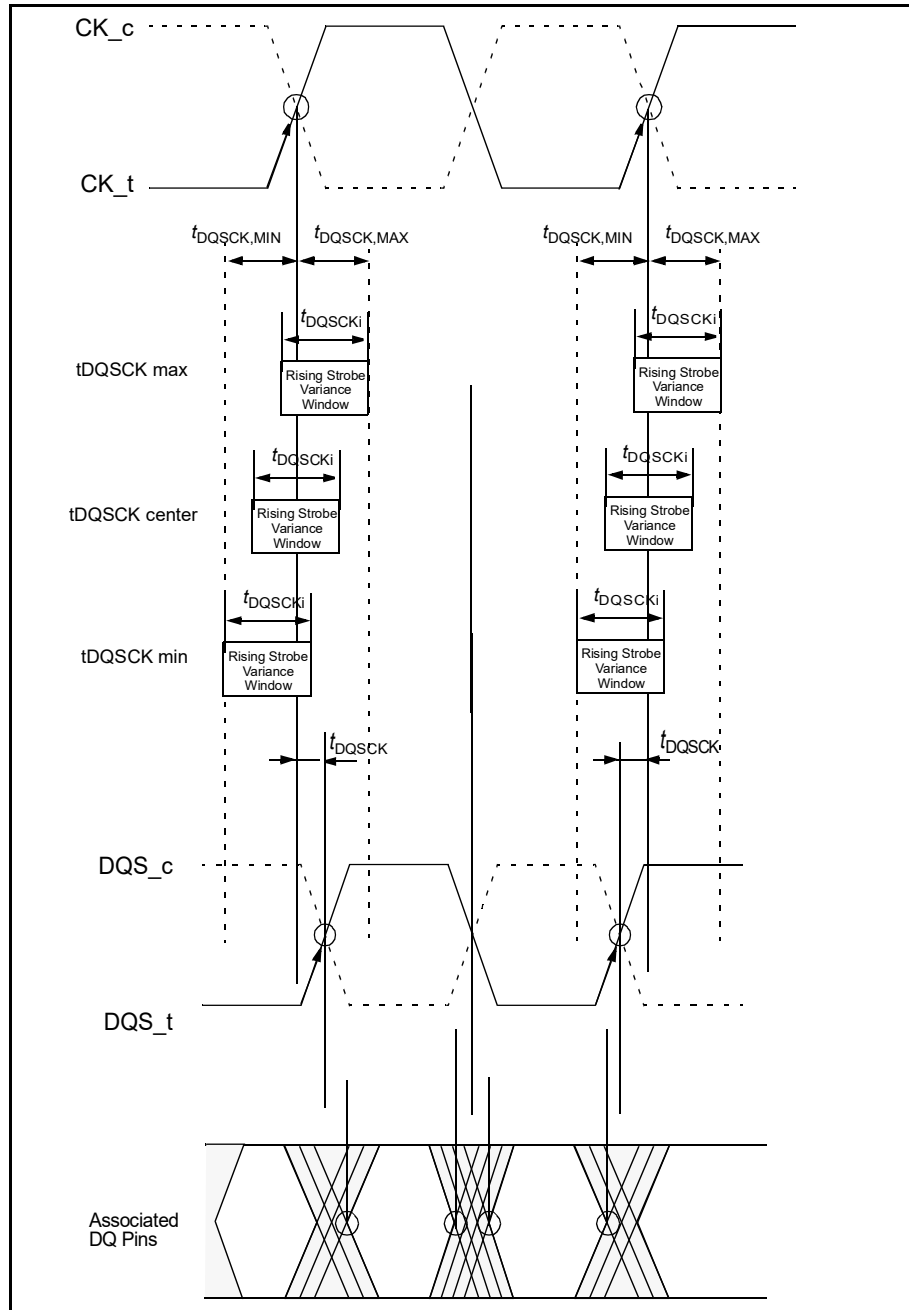
Figure 33 — TDQSCK Timing Definition
