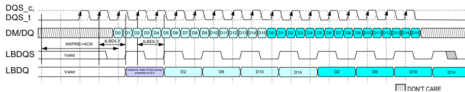
Figure 163 — Loopback Write Burst Output Mode 4-Way PhaseC Data Burst Bit and PhaseA Strobe Alignment WPRE=4CK Optional Example
