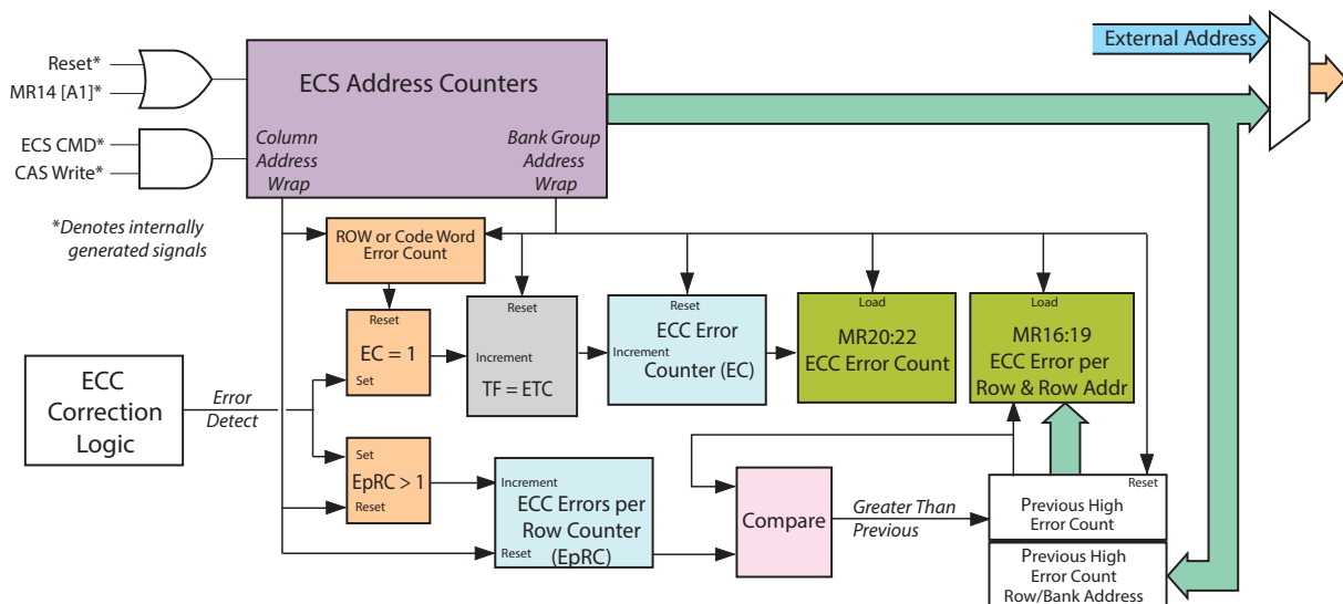
Figure 142 — Example of an ECC Transparency and Error Scrub Functional Block Diagram
