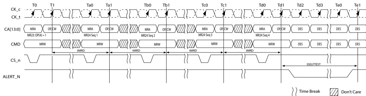
Figure 126 — MBIST Procedure
