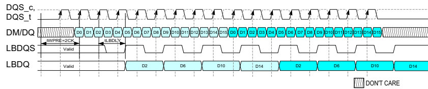
Figure 161 — Loopback Write Burst Output Mode 4-Way PhaseC WPRE=2CK Example
