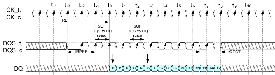
Figure 225 — Read burst example for pin DQx depicting bit 0 and 5 relative to the DQS edge for 2 UI skew with Read DQS Offset Timing set to 1 Clock (2UI)
