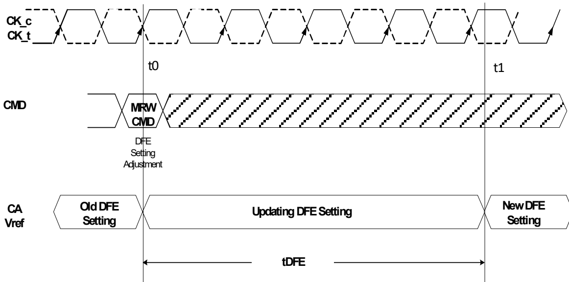
Figure 8 — DFE Update Setting
