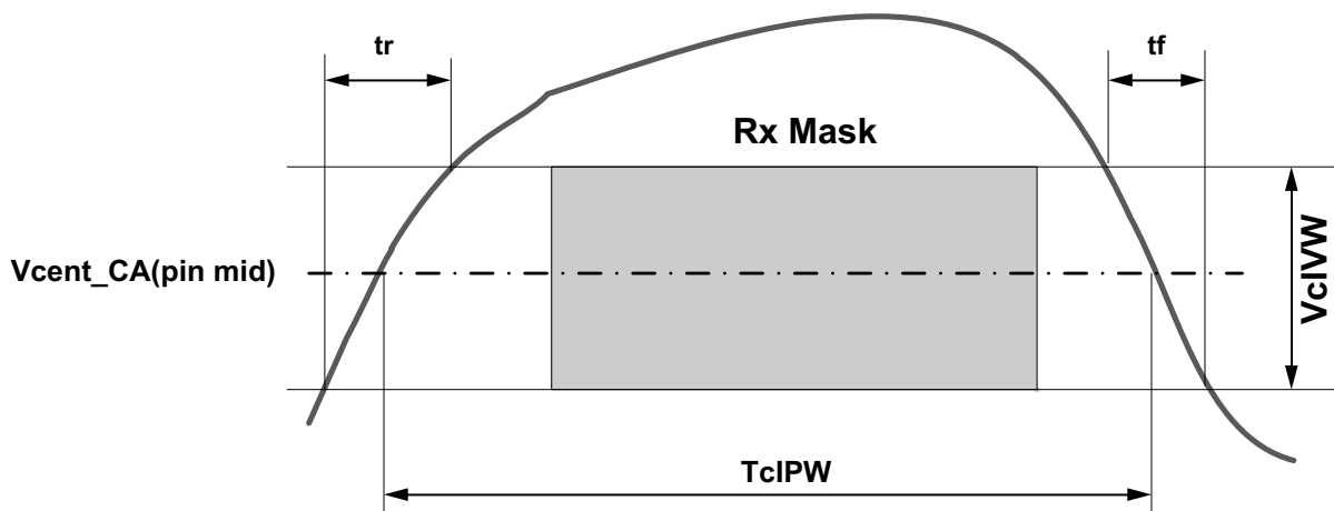
Figure 200 — CA TcIPW and SRIN_clVW definition (for each input pulse)
