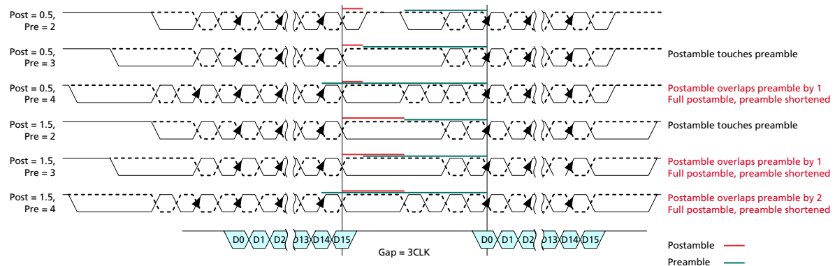
Figure 25 — Example of Consecutive Writes Operation: t_{CCD}=\text{Min}+3
