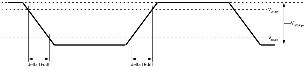
Figure 222 — Differential Output Slew Rate Definition
