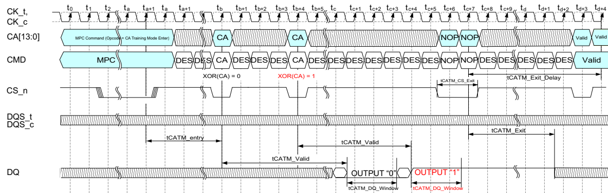
Figure 83 — Timing Diagram for CA Training Mode
