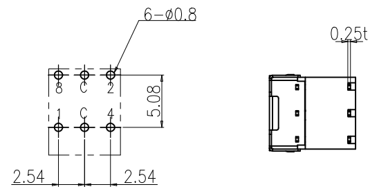
P.C.B DIMENSION (Top View)
