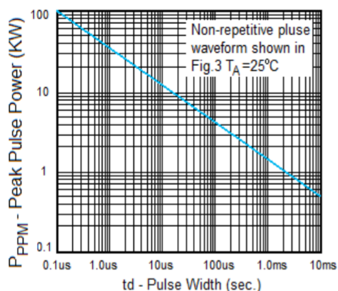
Fig. 1 Peak Pulse Power Rating
