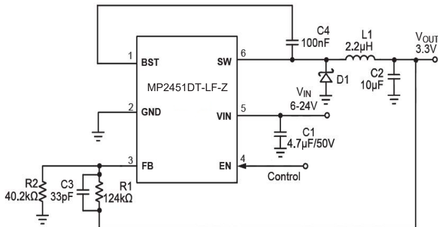
3.3V output typical application circuit
