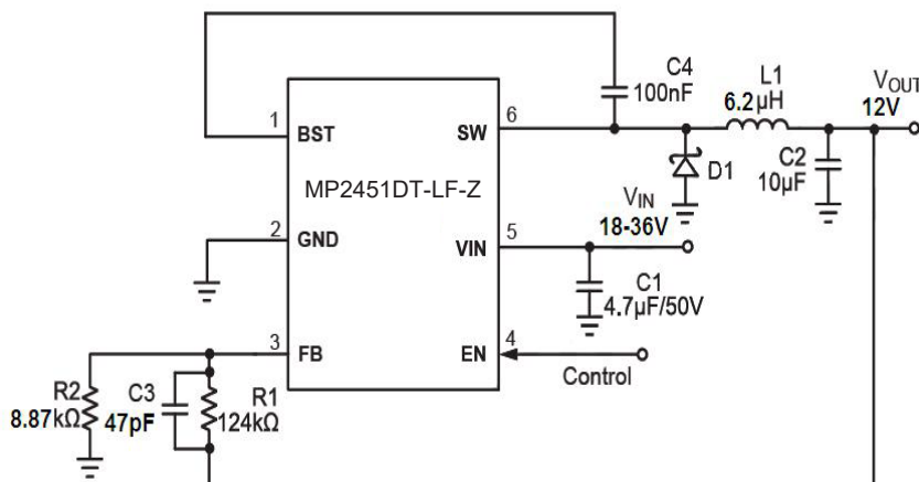
12V output typical application circuit
