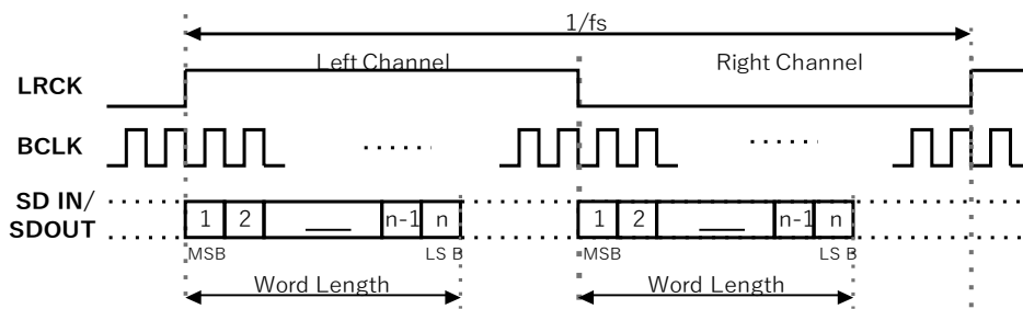
Left Justified mode (Offset=0)
