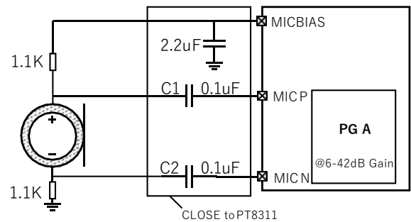
Differential Mic Input
