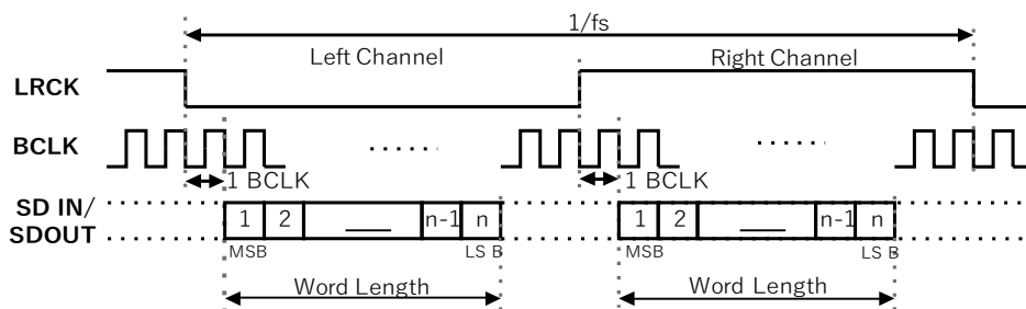
I2S standard mode (Offset=1)
