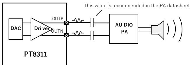
Line-out differential mode
