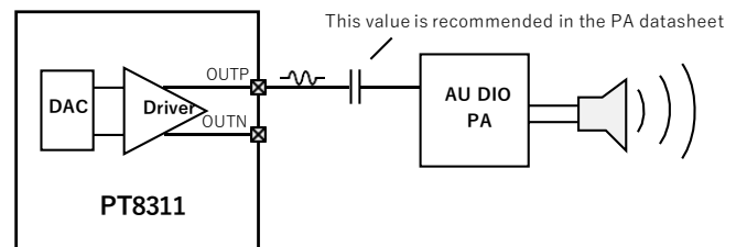
Line-out single-ended mode
