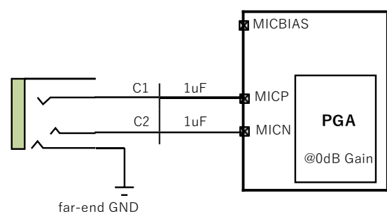
Differential Line-in
