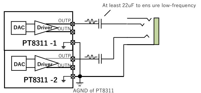
Headphone stereo mode
