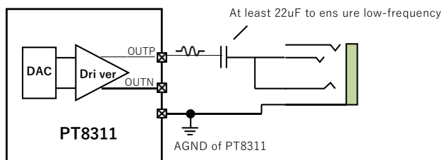
Headphone mono mode
