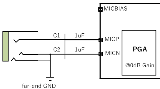
Single-Ended Line-in
