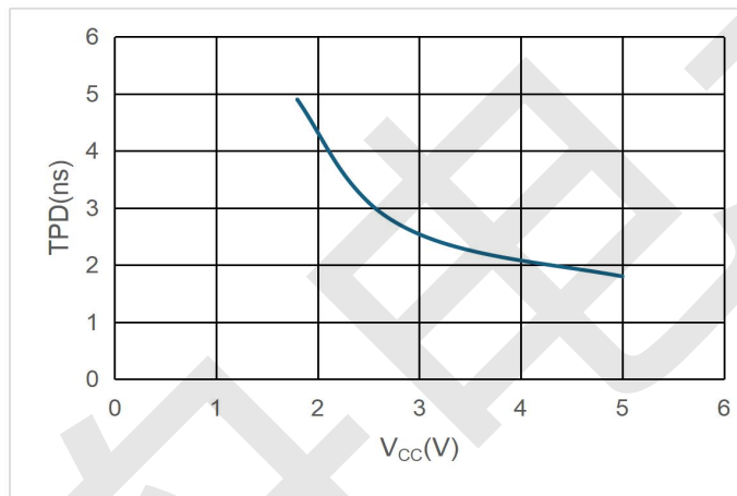
Figure 1. T_{PD} across V_{CC} at 25°C
