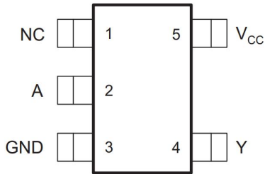
SOT23-5 and SOT353 (Top View)
