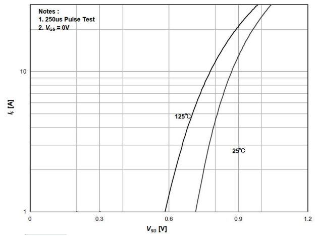
Figure 4. Body Diode Forward Voltage Variation with Current
