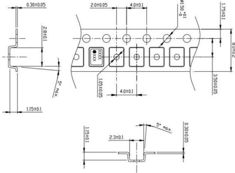
1. Clearance of an embossing tape, and a product unit: mm
