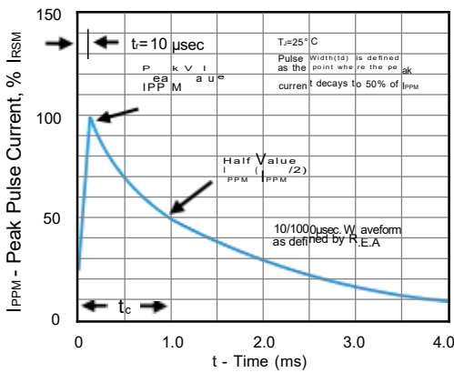
FIG.3-PULSE WAVE FORM
