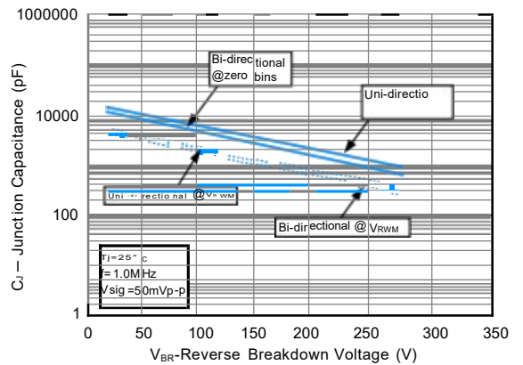
FIG.4-TYPICAL JUNCTION CAPACITANCE
