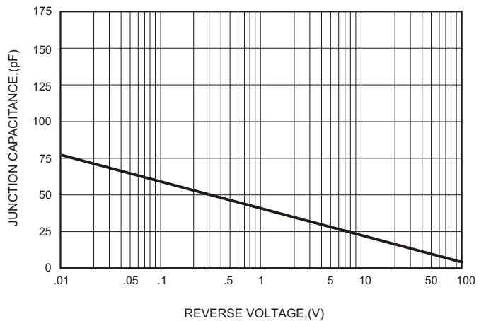
FIG.6-TYPICAL JUNCTION CAPACITANCE
