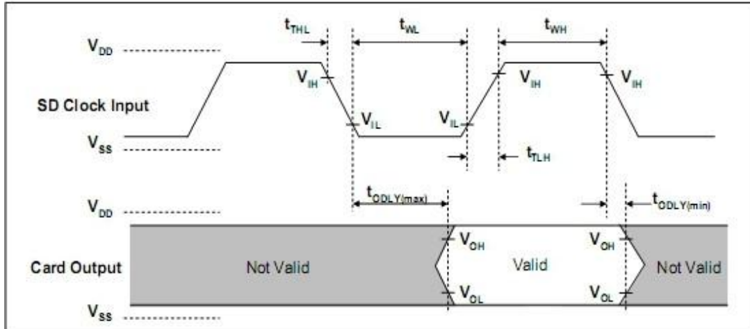
Figure 3: Card Output Timing (Default Speed Mode)
