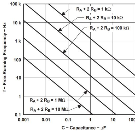
Figure 6. Free-Running Frequency
