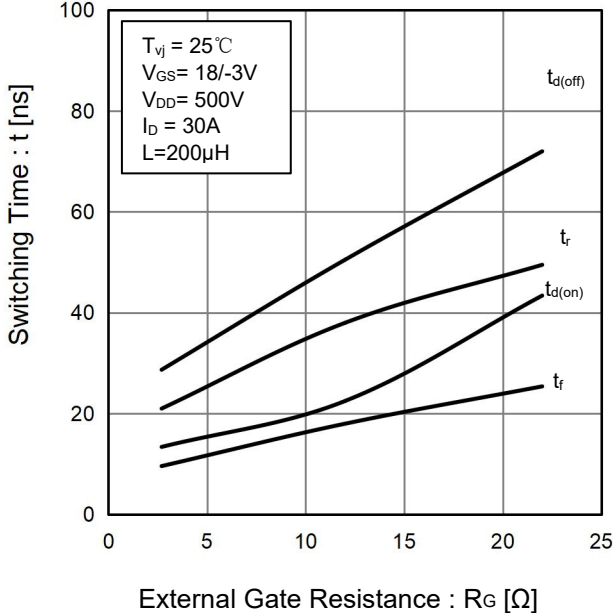
Fig.17 Typical Switching Time vs. External Gate Resistance
