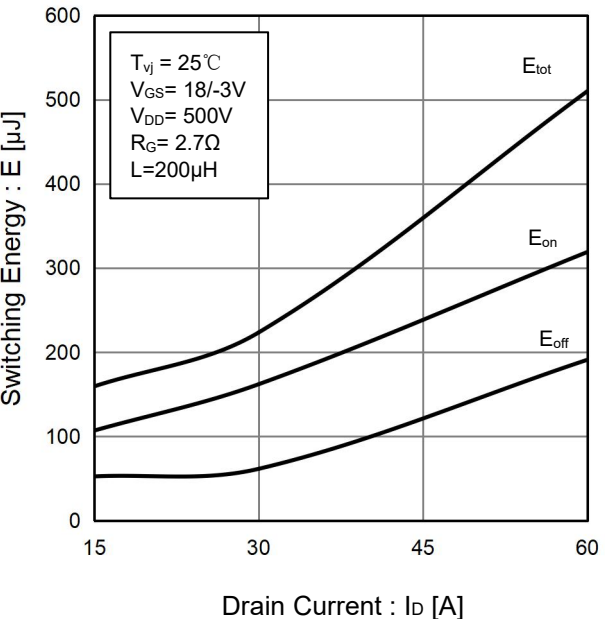
Fig.19 Typical Switching Energy vs. Drain Current
