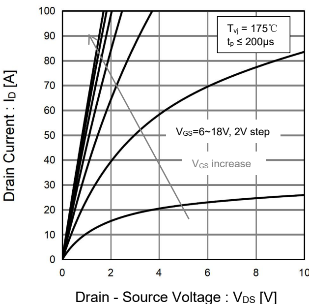
Fig.6 T_{vj} = 175^{\circ}\text{C} Typical Output Characteristics
