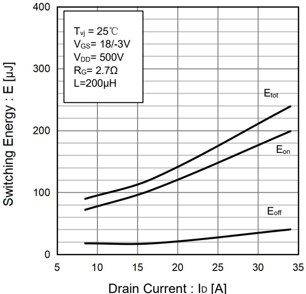
Fig.19 Typical Switching Energy vs. Drain Current
