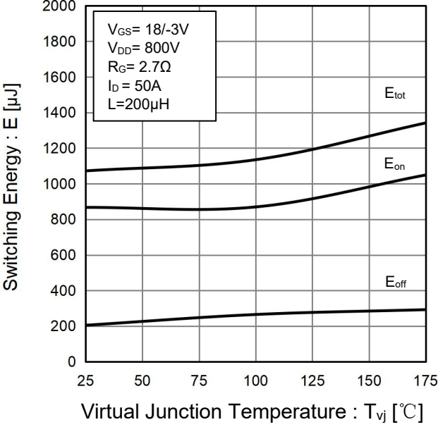
Fig.20 Typical Switching Energy vs. Virtual Junction Temperature
