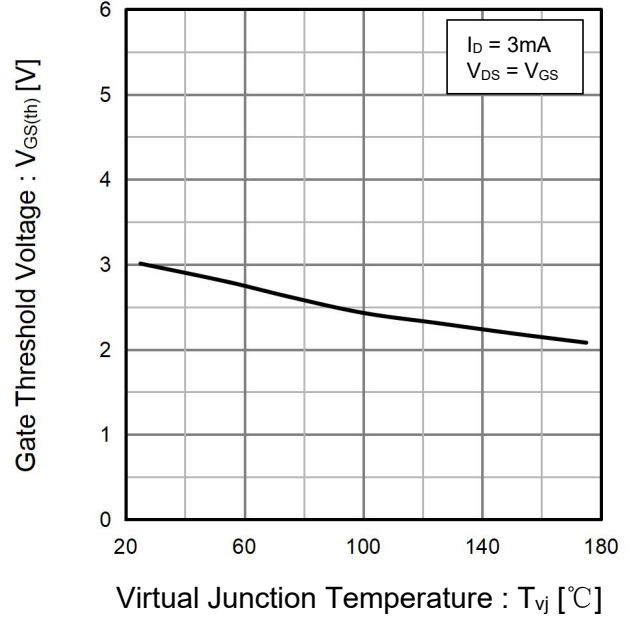
Fig.13 Gate Threshold Voltage vs. Virtual Junction Temperature
