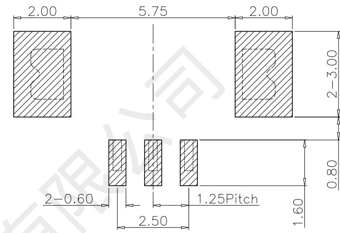
RECOMMENDER P.C.B LAYOUT TOP VIEW (GENERAL TOLERANCE ±0.10)
