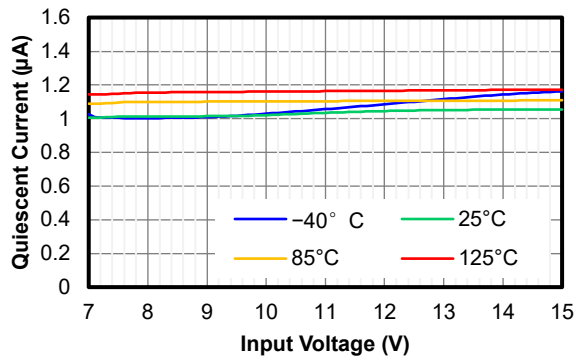
Figure 3. Quiescent Current vs. V_{IN}
