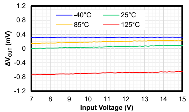
Figure 4. Line Regulation
