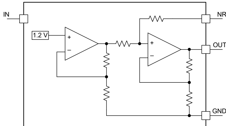
Figure 13. Functional Block Diagram
