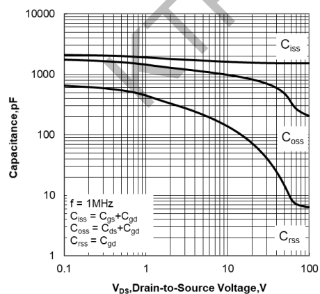
Figure 5. Capacitance Characteristics
