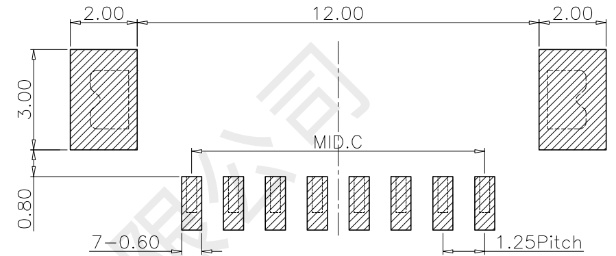
RECOMMENDER P.C.B LAYOUT TOP VIEW (GENERAL TOLERANCE ±0.10)
