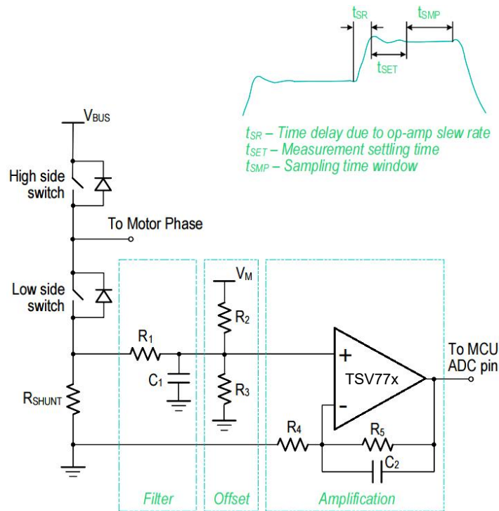
Figure 7. Current Shunt Monitor Circuit
