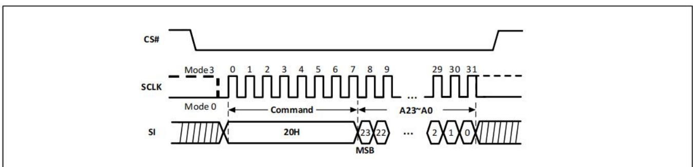
Figure-35. Sector Erase Sequence Diagram
