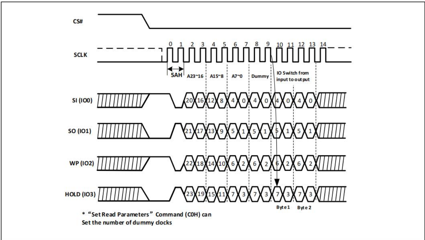
Figure-65. Read Serial Flash Discoverable Parameter Sequence Diagram (QPI)
