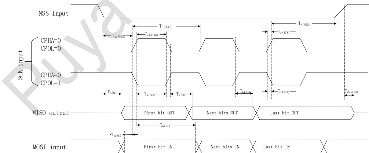
图 5-1 SPI 时序图—Slave mode and CPHA=0
