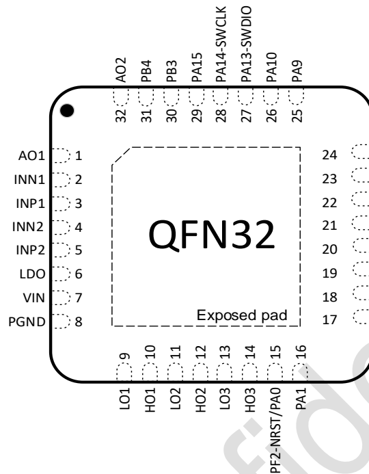
图 3-1 QFN32(4*4) Pinout1 PY32MD410K1xU (Top view)
