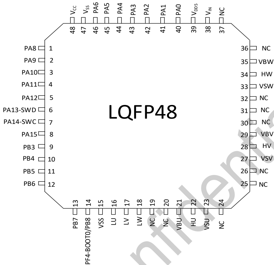
图 3-2 LQFP48 Pinout2 PY32MD540C2xT(Top view)
