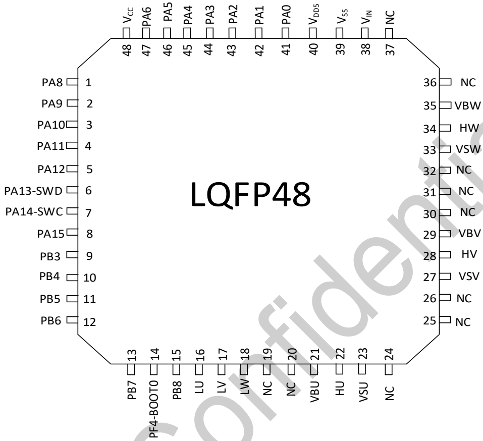
图 3-1 LQFP48 Pinout1 PY32MD540C1xT(Top view)
