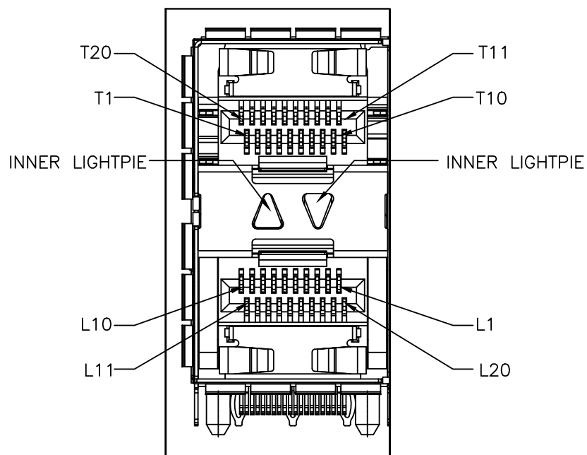
DETAIL A CIRCUIT NUMBERING AND LIGHTPIE INDENTIFICATION
