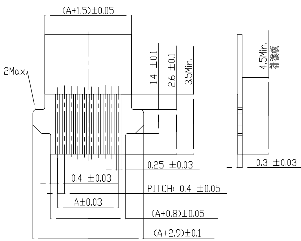
RECOMMEND FFC/FPC SCALE:5:1
