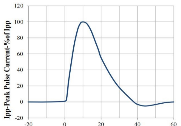
8 X 20us Pulse Waveform
