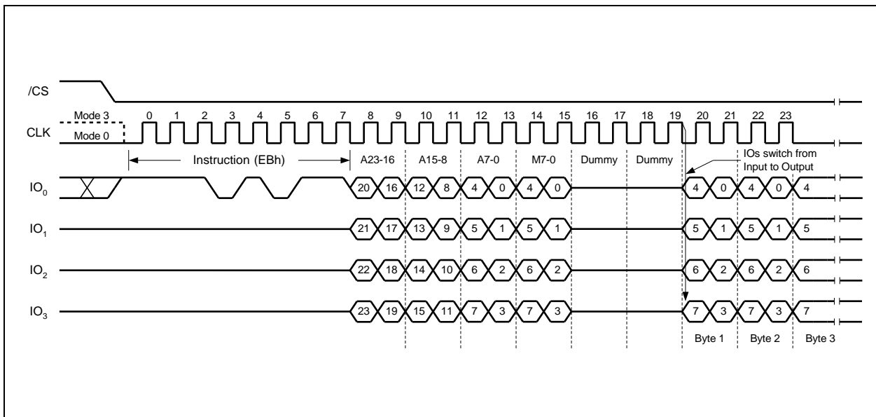
Figure 24a. Fast Read Quad I/O Instruction (Initial instruction or previous M5-4≠10, SPI Mode) "Set Read Parameters" instruction (C0h) can set the number of dummy clocks.
