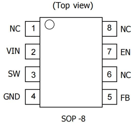
Figure 1. Pin Configuration of XBL1410 (Top View)
