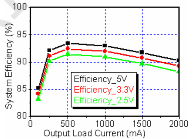
Figure 6. Efficiency vs. Load (Vin=10V)
