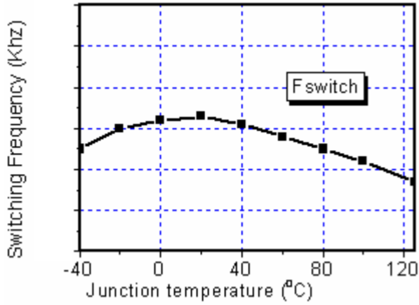
Figure 3. Switching Frequency vs. Temperature
