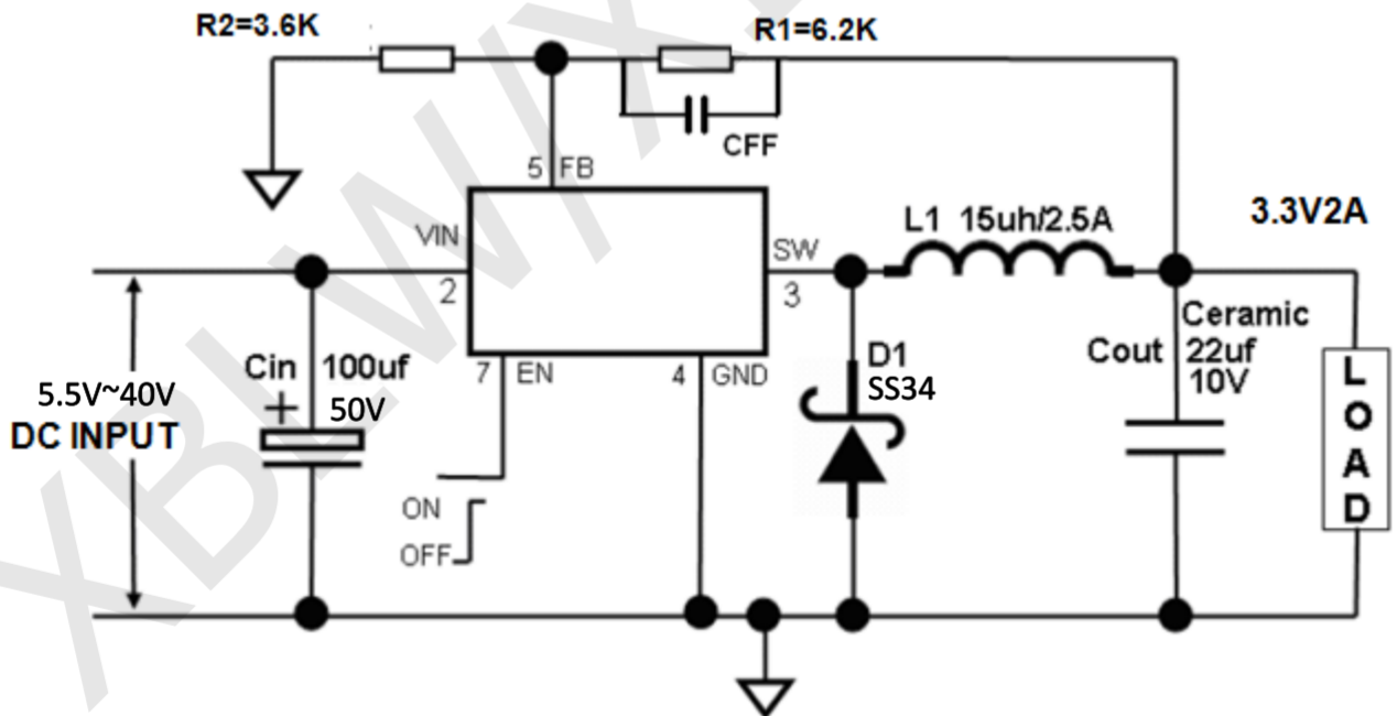
Fig 10. XBL1410 Typical Application Circuit (with ceramic output capacitor) @ 3.3V/2A
