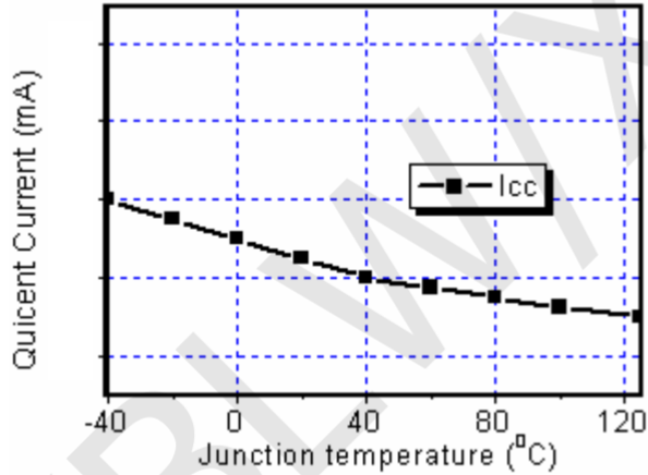
Figure 5. Icc vs. Temperature
