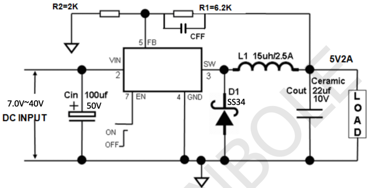
Fig 9. XBL1410 Typical Application Circuit (with ceramic output capacitor) @ 5V/2A
