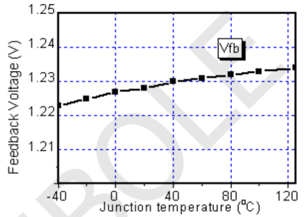
Figure 4. Vfb vs. Temperature
