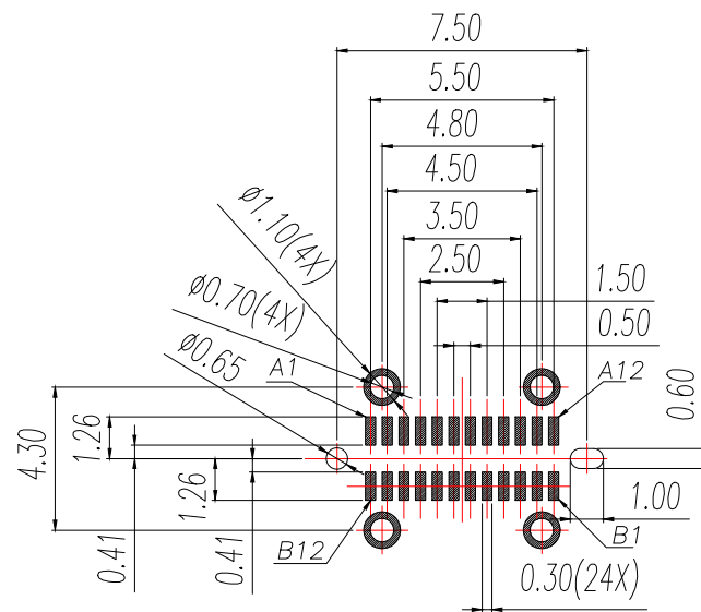
RECOMMENDED PCB LAYOUT(TOP VIEW) THICKNESS 1.0±0.10MM;DEFAULT TOLERANCE:±0.05
