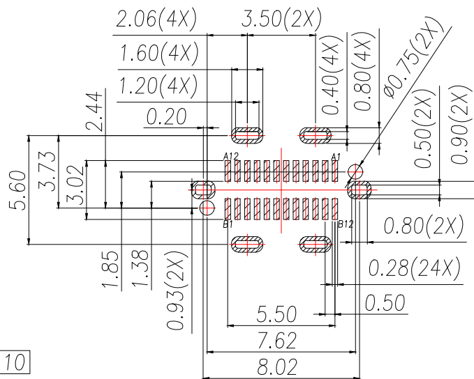
RECOMMENDED PCB LAYOUT(TOP VIEW) THICKNESS 0.8±0.10MM;DEFAULT TOLERANCE:±0.05
