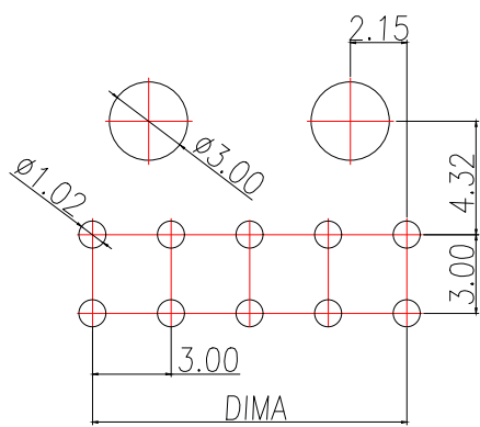
PCB.WELDING DRAWING (TOLERANCE:±0.05)
