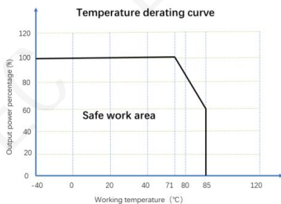
Figure 4: Temperature Derating Curve
