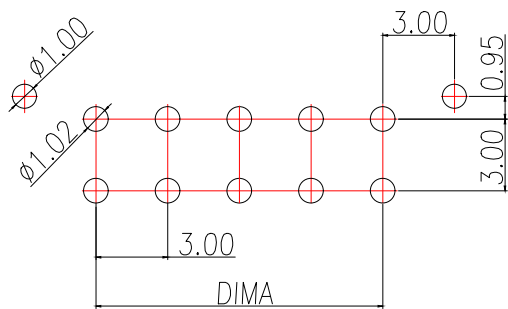
PCB WELDING DRAWING (TOLERANCE: \pm 0.05 )
