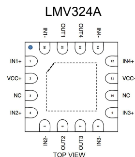
QFN-16 3*3
