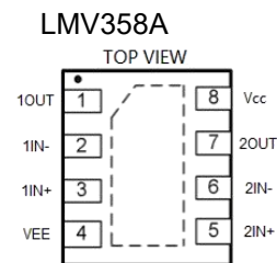
DFN-8 2*2/DFN-8 3*3
