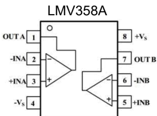
SOP-8/MSOP-8/DIP-8/TSSOP-8
