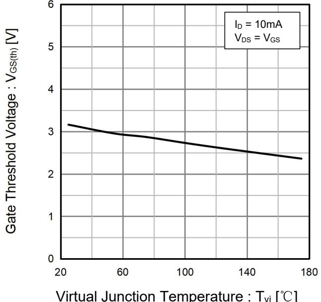
Fig.13 Gate Threshold Voltage vs. Virtual Junction Temperature
