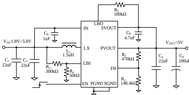
Figure 1. Schematic Diagram
