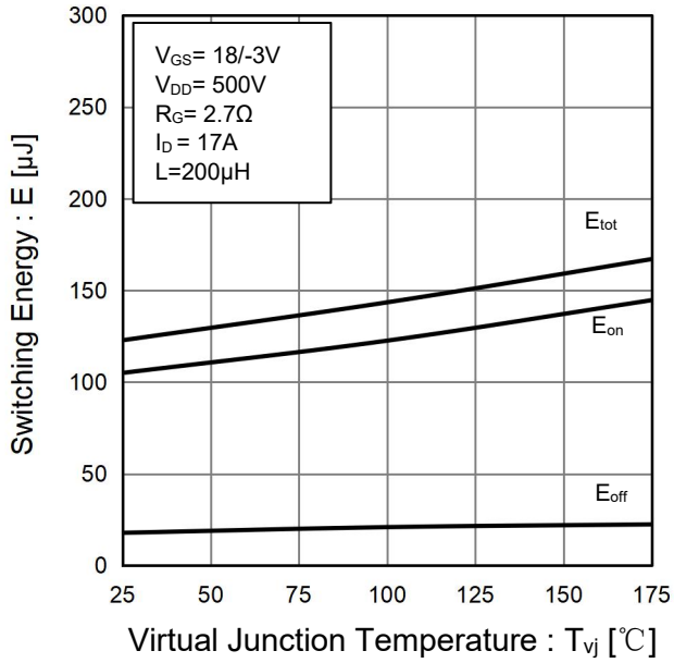
Fig.20 Typical Switching Energy vs. Virtual Junction Temperature
