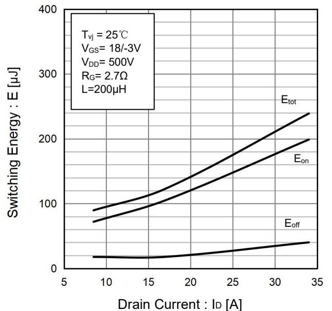
Fig.19 Typical Switching Energy vs. Drain Current
