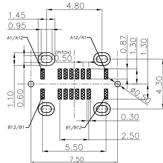
RECOMMENDED P.C.B. LAYOUT TOLERANCE UNSPECIFIED ±0.05mm
